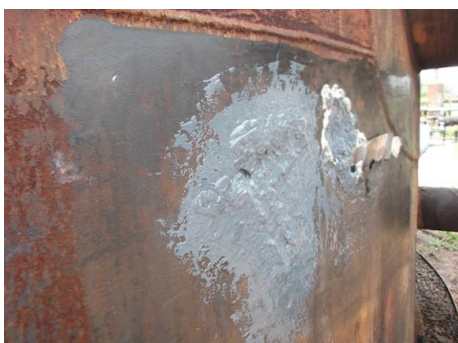
Repair works with SealXpert™ Repair Putty
